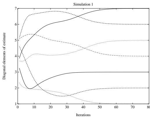
FIG. 2. A plot of the diagonal elements, h_{ii} , of each iteration, H_k , of the Lie-bracket algorithm run on a 7 \times 7 initial condition H_0 with eigenvalues (1, \dots, 7) . The target matrix N was chosen to be \text{diag}(1, \dots, 7) .
